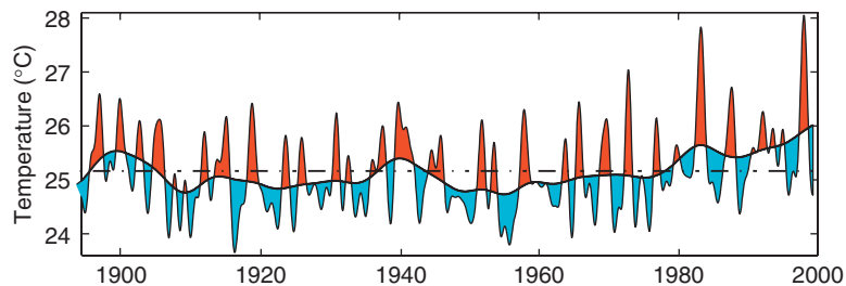
Figure 3 Interannual variations in sea surface temperatures (SSTs) in the eastern equatorial Pacific shown on the background of decadal changes (in ^{\circ} C). The annual cycle and high-frequency variations are removed from the data. El Niño conditions correspond to warmer temperatures. Note El Niño events of 1982 and 1997, the strongest in the instrumental record. From Fedorov AV and Philander SG (2000) Is El Niño changing? Science 288: 1997–2002.
