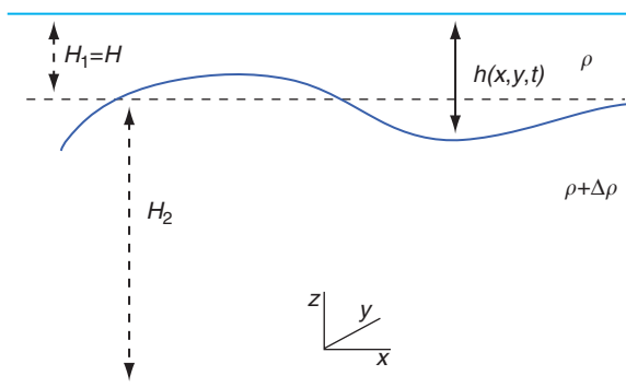
Figure 5 A sketch of the 1\frac{1}{2} -layer shallow-water system with the rigid-lid approximation. H_1/H_2 \ll 1 . The mean depth of the thermocline is H . The x -axis is directed to the east along the equator. The y -axis is directed toward the North Pole. The mean east–west thermocline slope along the equator is neglected.
