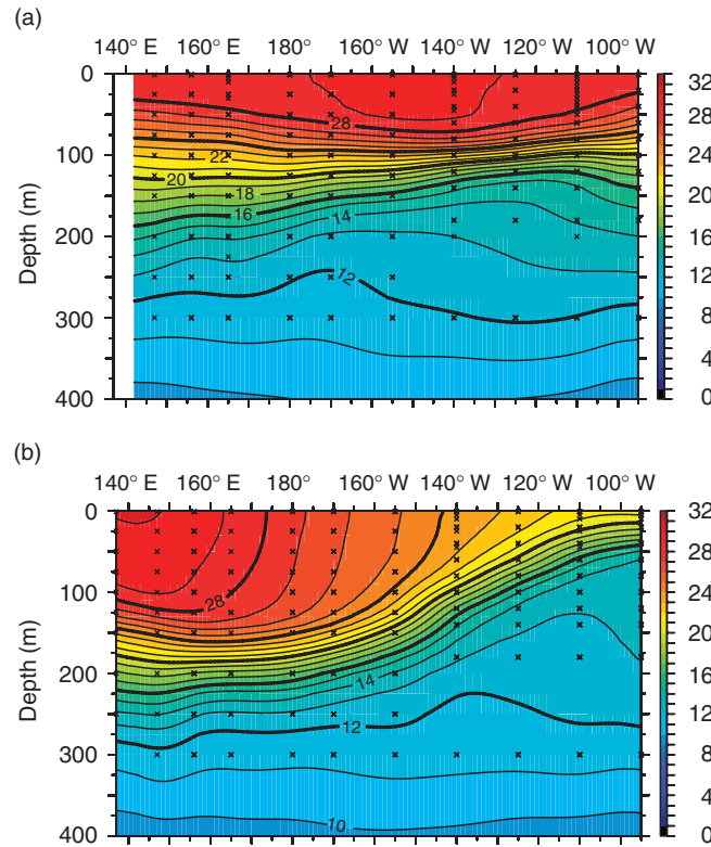
Figure 4 Temperatures ( ^{\circ}\text{C} ) as a function of depth along the equator at the peaks of (a) El Niño (Jan. 1998) and (b) La Niña (Dec. 1999). From the TAO data; see McPhaden MJ (1999) Genesis and evolution of the 1997–98 El Niño. Science 283: 950–954.
