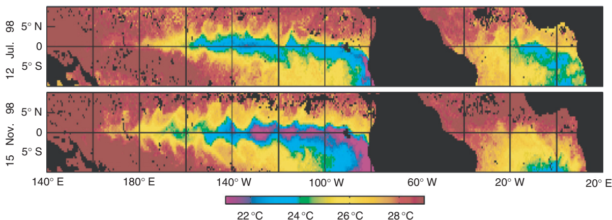
Figure 17 Tropical instability waves (TIWs): 3-day composite-average maps from satellite microwave SST observations for the periods 11–13 July 1998 (upper) and 14–16 November 1998 (lower). Black areas represent land or rain contamination. The waves propagate westward at approximately 0.5 \text{ m s}^{-1} . From Chelton DB, Wentz J, Gentemann CL, de Szoeke RA, and Schlax MG (2000) Satellite microwave SST observations of trans-equatorial tropical instability waves. Geophysical Research Letters 27(9): 1239–1242.
