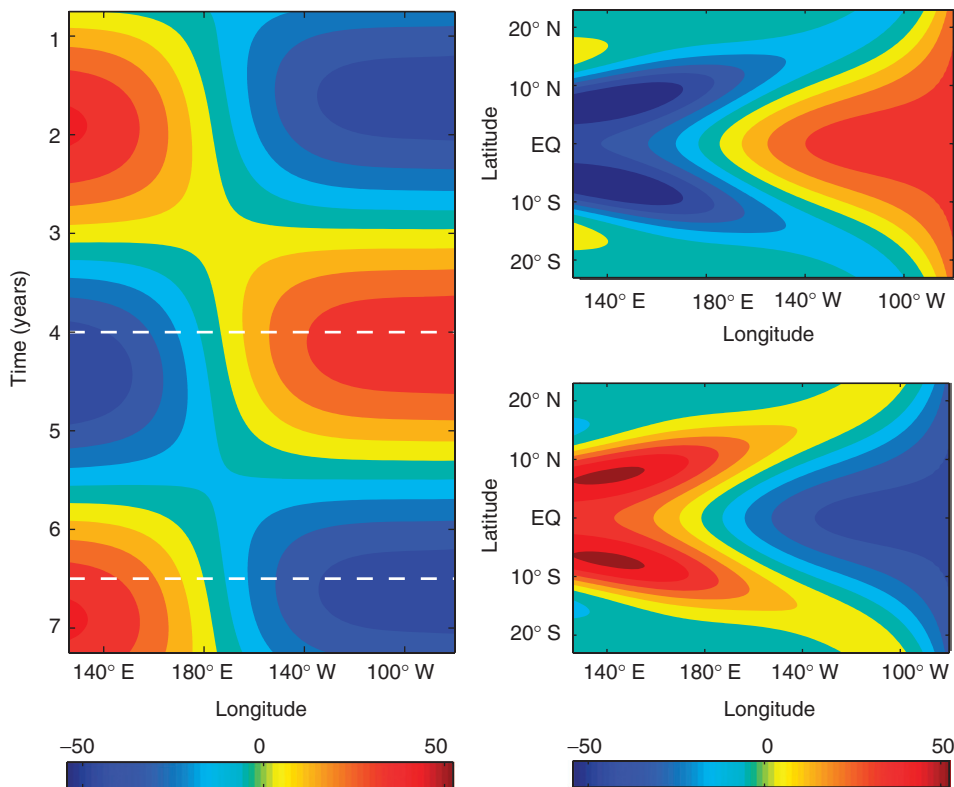
Figure 9 Ocean response to oscillatory winds in a shallow-water model. Left: a Hovmoller diagram of the thermocline depth anomalies along the equator. Note the different temporal scale as compared to Figure 8 . Right: the spatial structure of the anomalies at times indicated by the dashed lines on the left-side panel. Red corresponds to a deeper thermocline, blue to a shallower thermocline. The wind-stress anomaly is calculated as \tau = \tau_0 \sin(2\pi t/P) \exp[-(x/L_x)^2 - (y/L_y)^2] ; P = 5 years.
