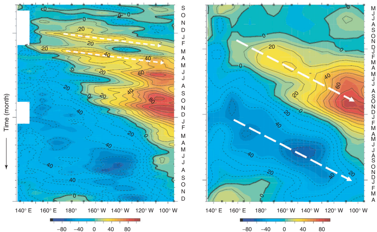
Figure 15 Observations of Kelvin waves and El Niño from the TAO array. Anomalies with respect to the long-term average of the depth of the 20^\circ\text{C} -degree isotherm are shown before and after the development of El Niño of 1997. Left: 5-day averages; the time axis starts in September 1996. Right: monthly averages; the time axis starts in May 1996 (cf. Figures 8 and 9 ). The dashed lines in the left-side panel correspond to Kelvin waves excited by brief WWBs and rapidly traveling across the Pacific. The dashed lines in the right-side panel show the slow eastward progression of warm and cold temperature anomalies associated with El Niño followed by a La Niña. The monthly averaging effectively filters out fast Kelvin waves from the picture leaving only gradual interannual changes. It has been argued that the Kelvin waves may have contributed to the exceptional strength of El Niño in 1997–98.
