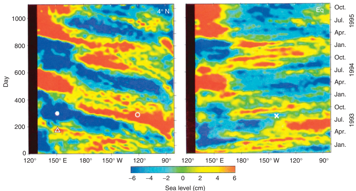
Figure 13 Observations of Rossby (left) and Kelvin (right) waves. Time-longitude sections of filtered sea level variations in the Pacific Ocean along 4^\circ N and along the equator are shown. A section along 4^\circ S would be similar to the 4^\circ N section. The symbols (x, triangle, and circles) correspond to the times and locations of the matching symbols in Figure 14. Note that time runs from bottom to top. Obtained from TOPEX/POSEIDON satellite data; from Chelton DB and Schlax MG (1996) Global observations of oceanic Rossby Waves. Science 272(5259): 234–238.
