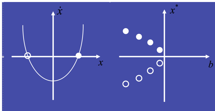
Figure 1: Saddle-node bifurcation diagram using the graphical method.
