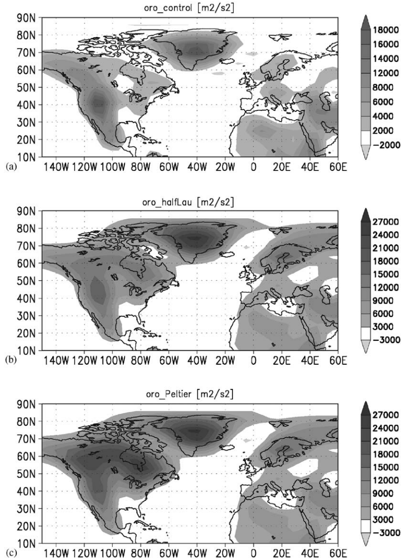
Fig. 1. Surface geopotential ( \text{m}^2 \text{s}^{-2} ) for: (a) the control run; (b) the exp. with half of the height of the Laurentide Ice Sheet; (c) the exp. with full height of the Laurentide Ice Sheet.
