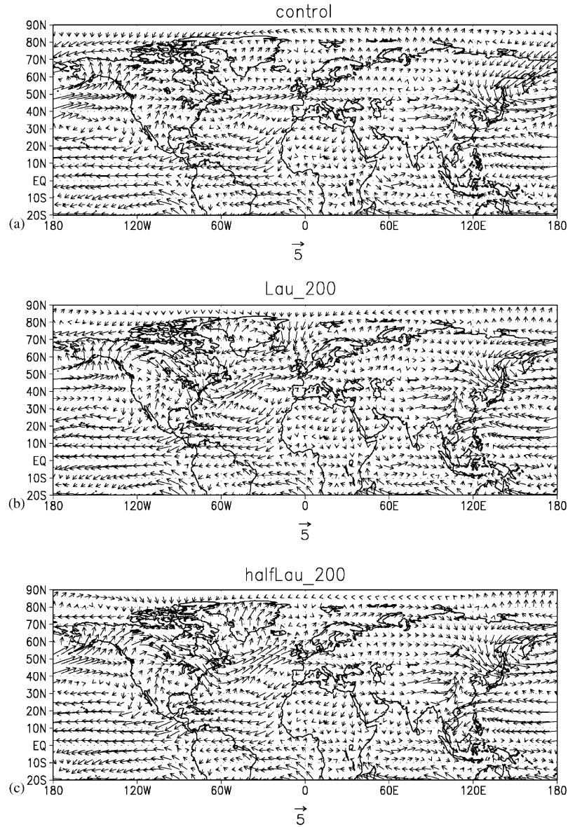
Fig. 8. Surface wind field for (a) control run; (b) Lau_200 and (c) halfLau_200 experiments. The fields are averaged over 25 years of integration. Units are \text{ms}^{-1} .
