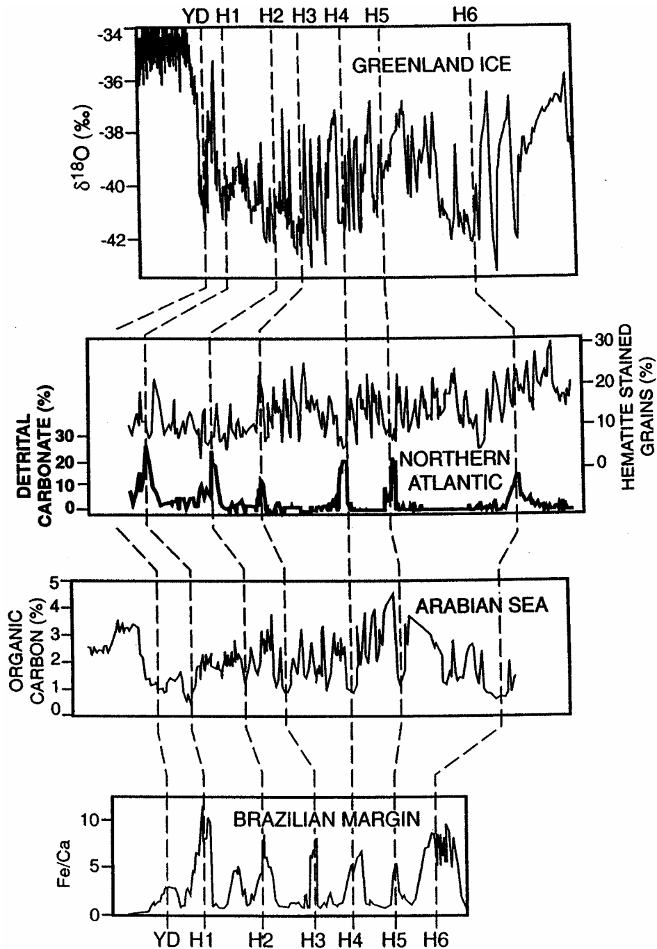
Figure 49. Comparison of four records showing a range in the ratio of the climatic impacts of Heinrich events to those of Dansgaard-Oeschger events. On the top is the Summit Greenland \delta^{18}\text{O} record in which DO events dominate. In the center are records of ice rafting in the northern Atlantic Ocean (Bond et al., 1999) and of organic matter in the Arabian Sea (Schulz et al., 1998). In these records, the impacts of both H and DO events are apparent. At the bottom is the record of lithic input off Brazil in which only Heinrich events are seen (Arz et al., 1998). Time and depth scales are deliberately left off, but the Heinrich events are approximately 16, 22, 30, 38, 45, 65 ka.
