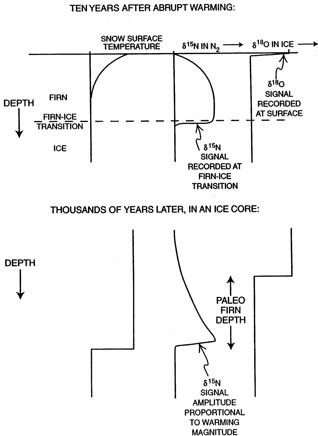
Figure 35. The imprint of an abrupt rise in air temperature on the ^{18}\text{O} to ^{16}\text{O} ratio in the ice and ^{15}\text{N} to ^{14}\text{N} ratio in the \text{N}_2 trapped in bubbles. The former is imprinted at the top of the firn and the latter is imprinted at the base of the firn. The enrichment of ^{15}\text{N} is the result of the thermal gradient in the firn. This ^{15}\text{N} enrichment gradually diminishes as the firn temperature equilibrates with that in the atmosphere but its imprint in the bubbles remains. The offset in depth between the ^{18}\text{O} change and the ^{15}\text{N} change records the paleothickness of the firn. By counting the number of annual layers in this interval, it is possible to determine the time offset between the gas record and ice record.
